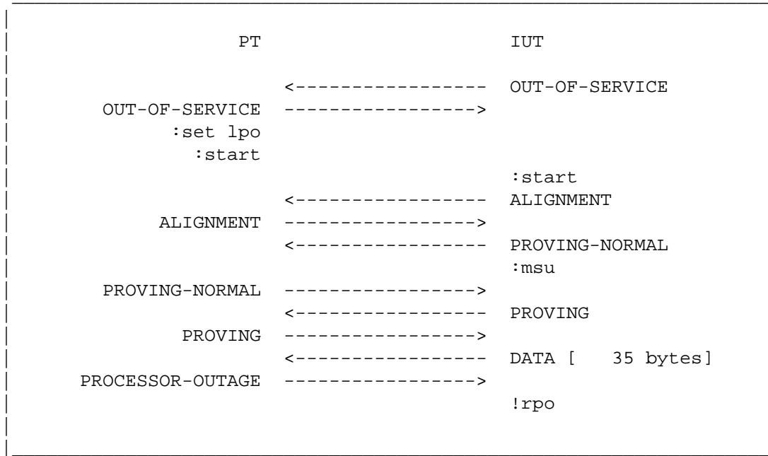
Figure 3.1.9-2. Normal alignment with PO set (Data)
