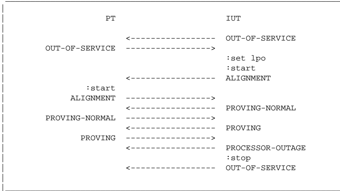
Figure 3.1.27-1. Deactivate during aligned not ready
