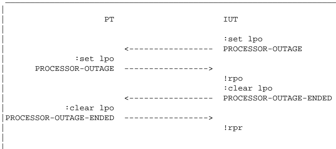
Figure 3.4.3-1. Clear LPO when "Both processor outage"
