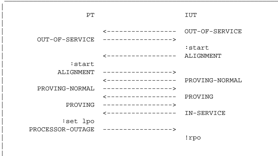
Figure 3.1.35-1. "Processor Outage" instead of "In Service"
