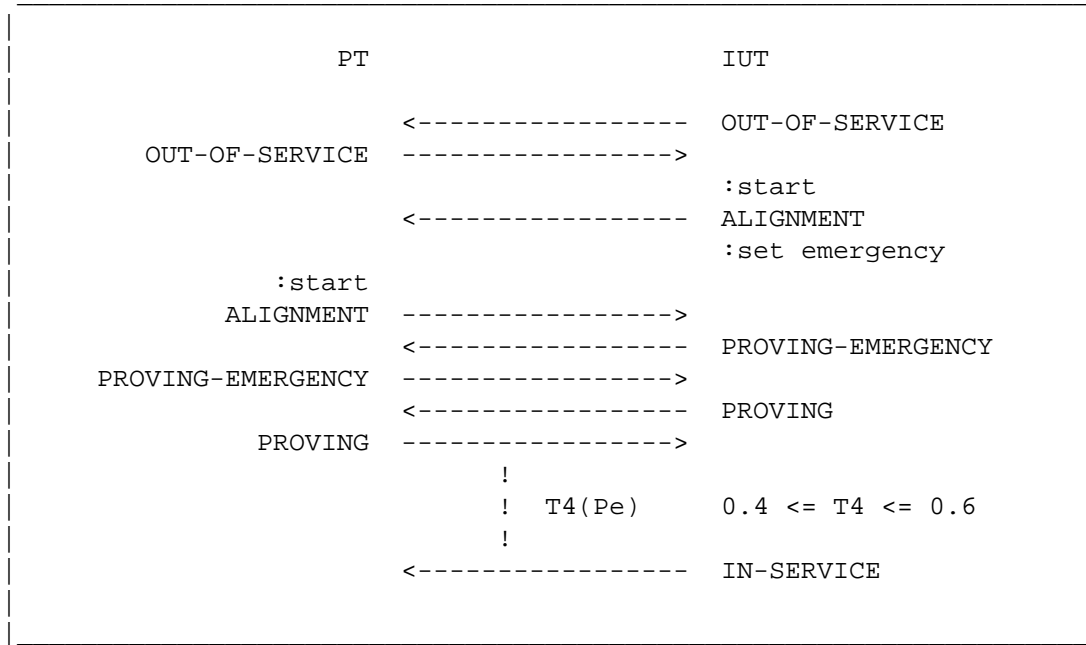
Figure 3.1.19-1. Set emergency in "not aligned" state
