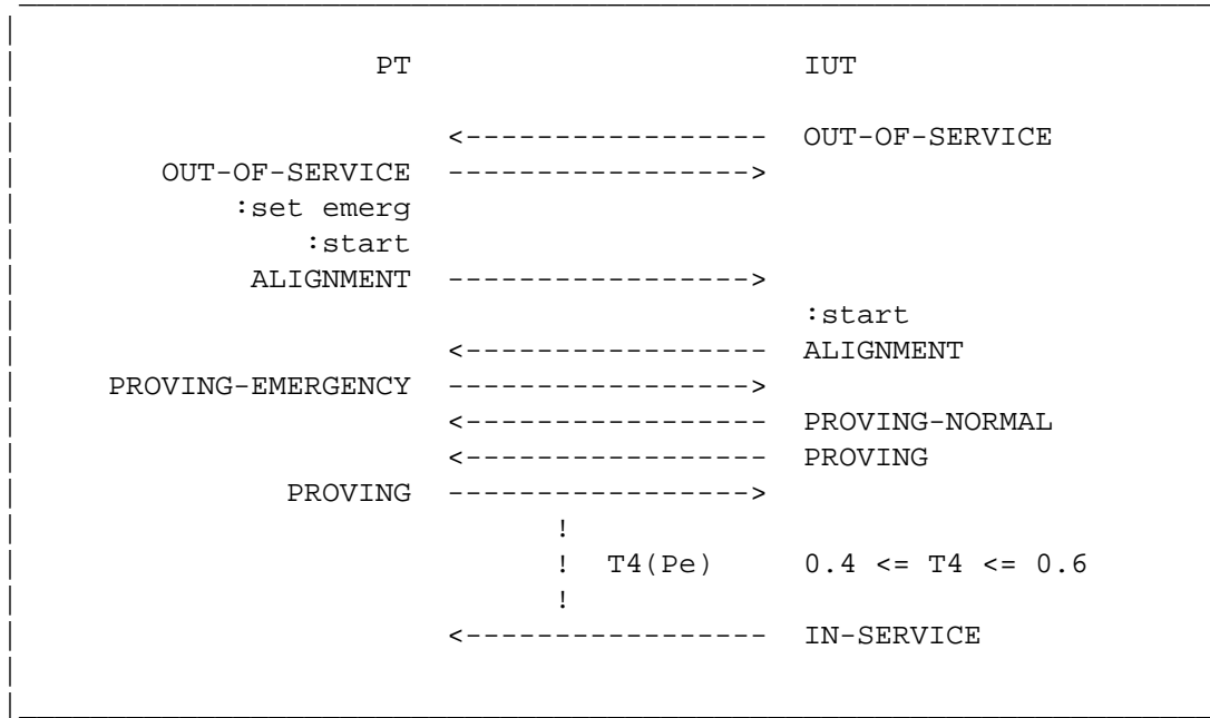
Figure 3.1.22-1. Individual end sets emergency
