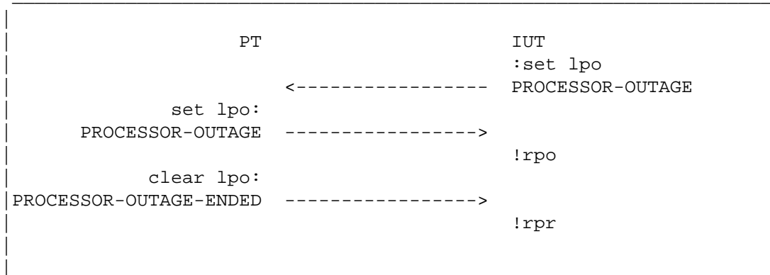
Figure 3.4.2-1. RPO during LPO
