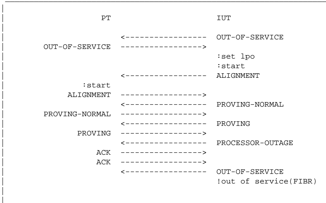
Figure 3.3.4-1. Link aligned not ready (Invalid Acks)
