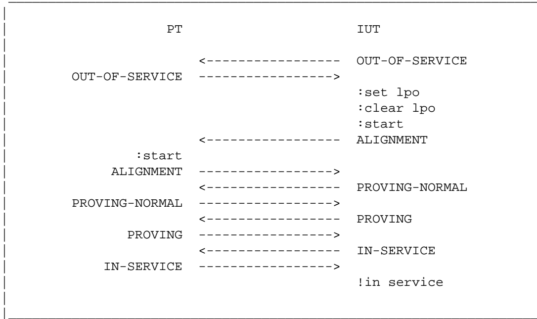
Figure 3.1.10-1. Normal alignment with PO set and cleared
