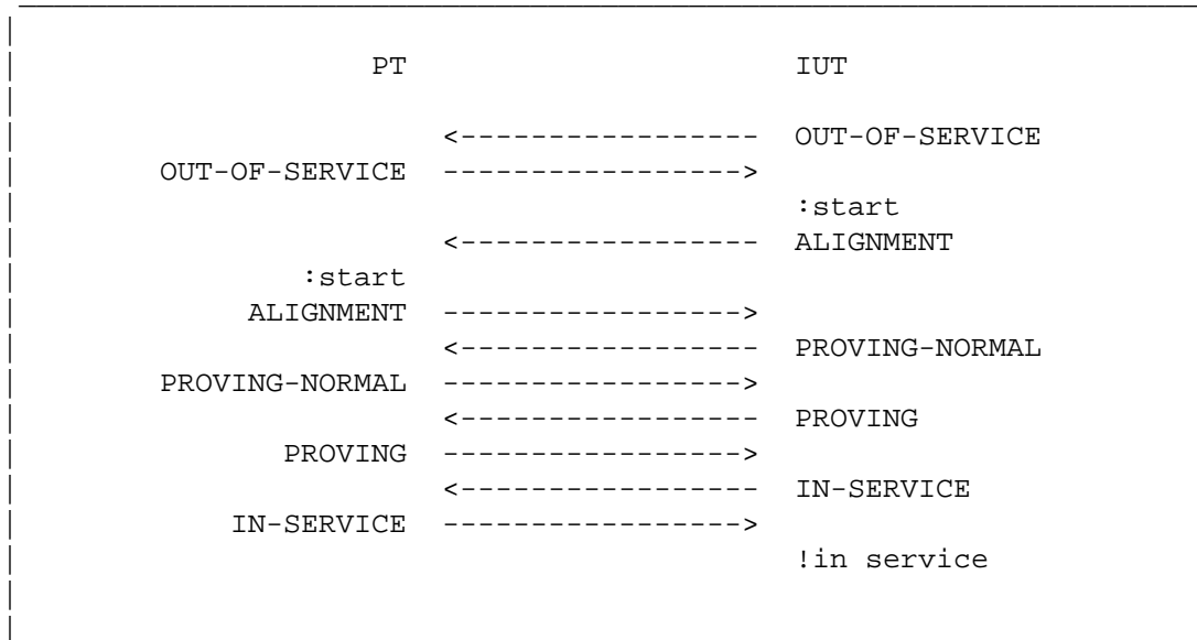
Figure 3.1.5-1. Normal alignment procedure
