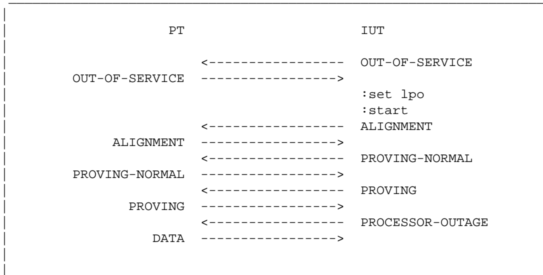
Figure 3.1.9-1. Normal alignment with PO set (Data)
