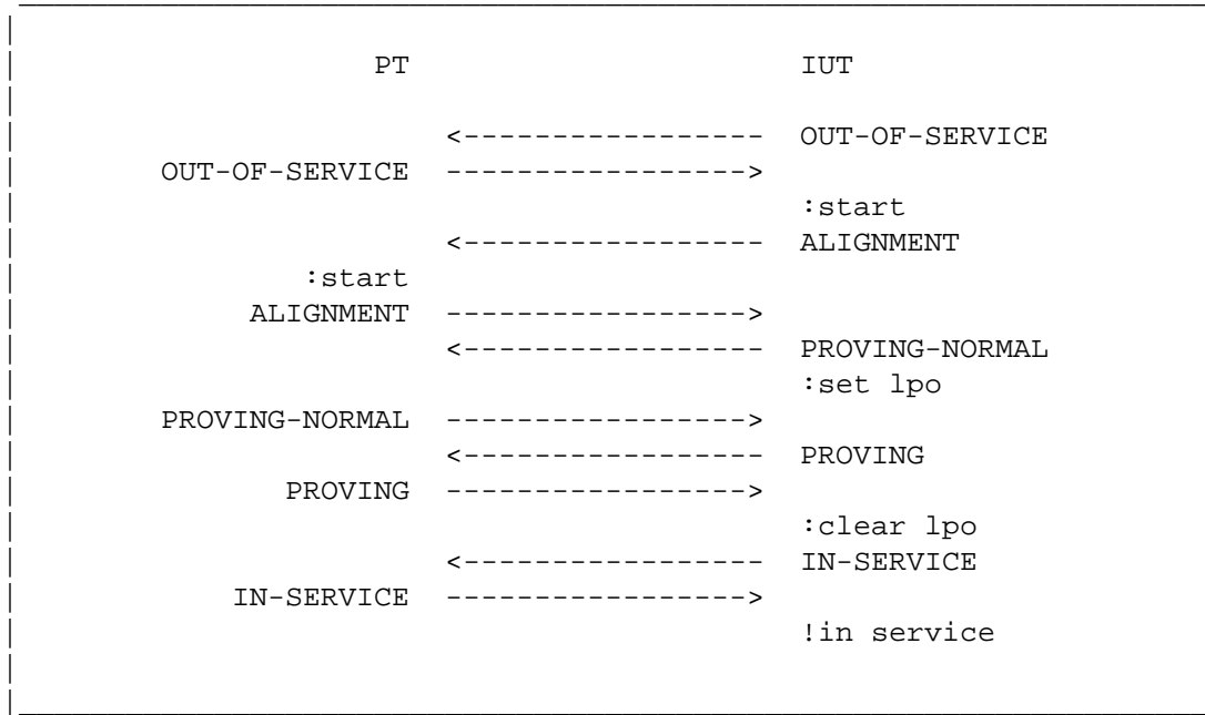
Figure 3.1.14-1. Set and clear LPO when "Initial Alignment"
