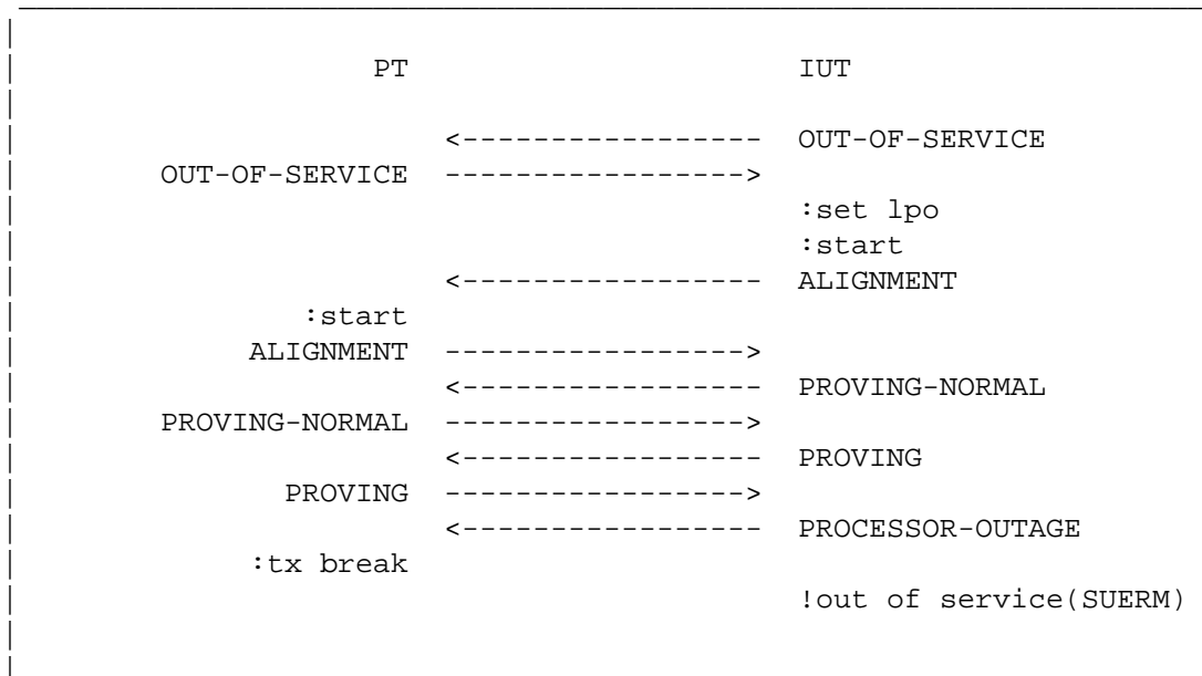
Figure 3.3.3-1. Link aligned not ready (Abort)
