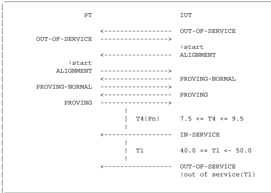
Figure 3.1.4-1. Timer T1 & Timer T4 (Normal)
