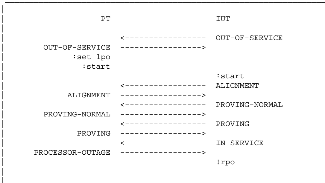
Figure 3.1.8-2. Normal alignment with PO set
