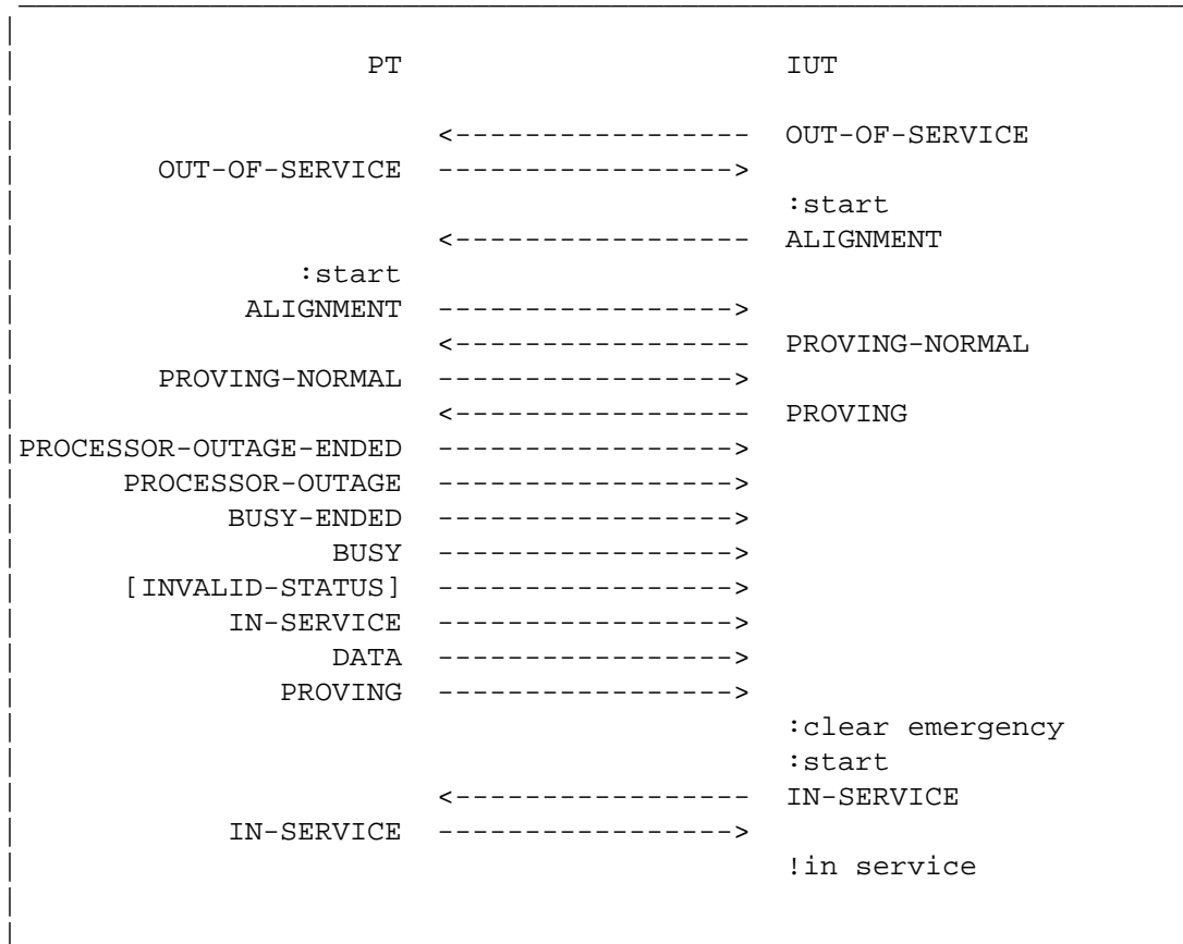
Figure 3.2.4-1. Unexpected events while "proving"
