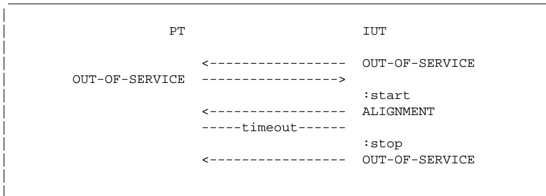
Figure 3.1.25-1. Deactivate during initial alignment
