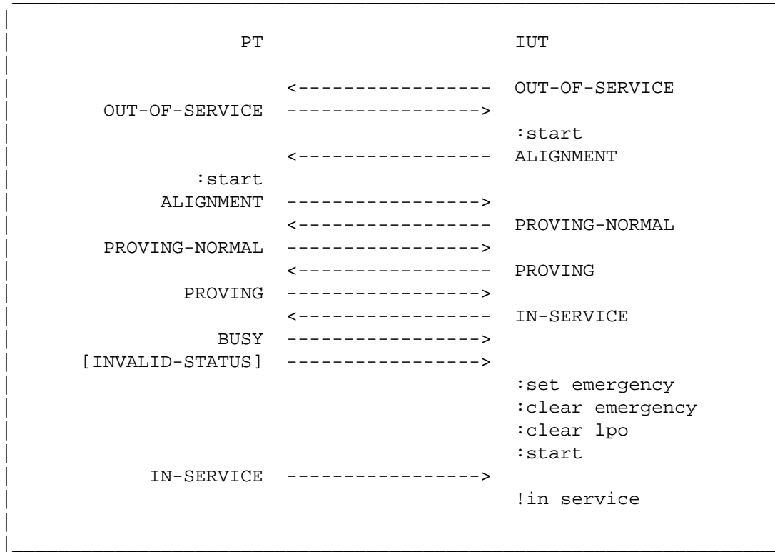
Figure 3.2.5-1. Unexpected events while "aligned ready"
