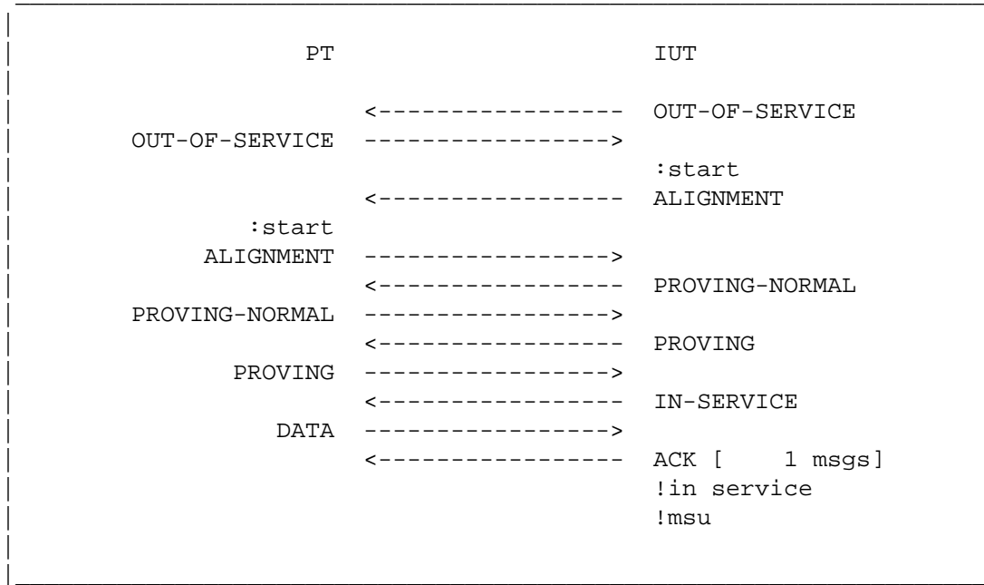
Figure 3.1.6-1. Normal alignment procedure (Data)
