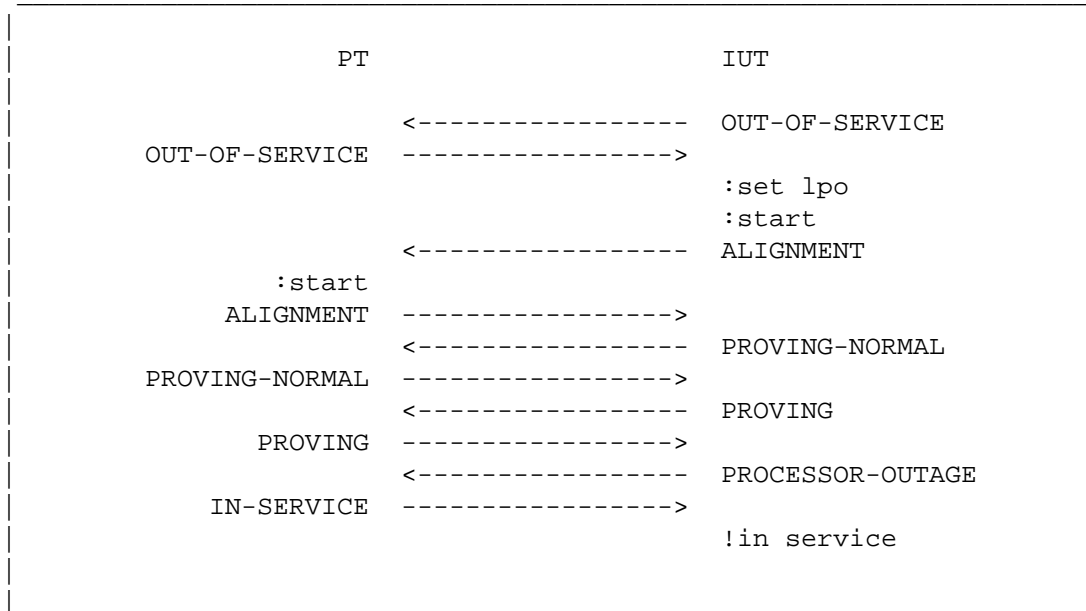
Figure 3.1.8-1. Normal alignment with PO set
