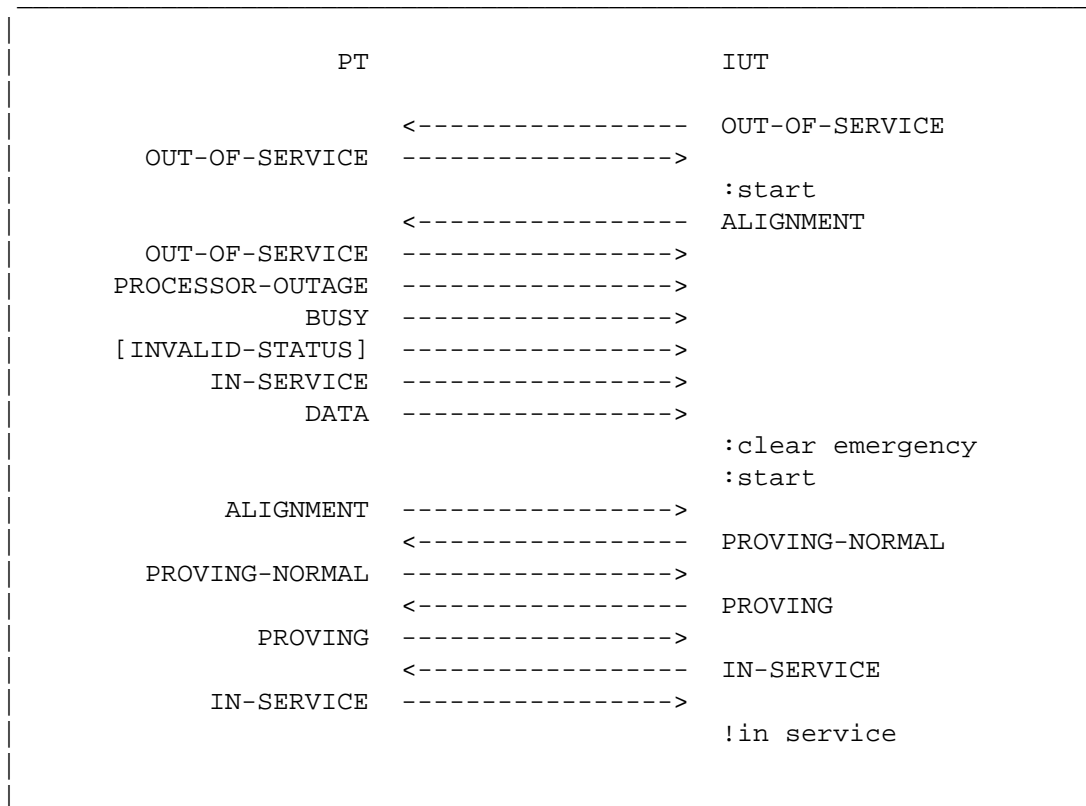
Figure 3.2.2-1. Unexpected events while "not aligned"
