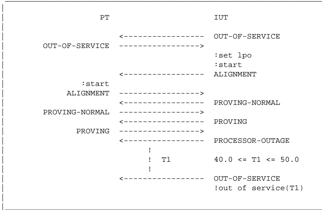
Figure 3.1.16-1. Timer T1 in "Aligned not ready" state
