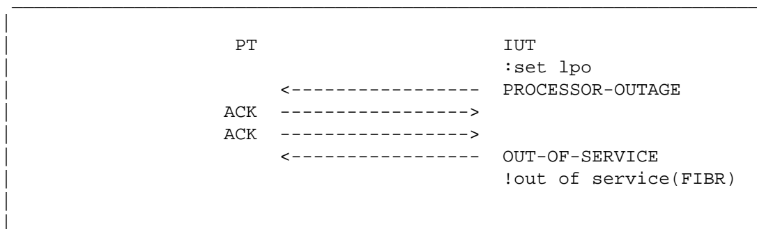
Figure 3.3.8-1. Link in processor outage (Invalid Acks)
