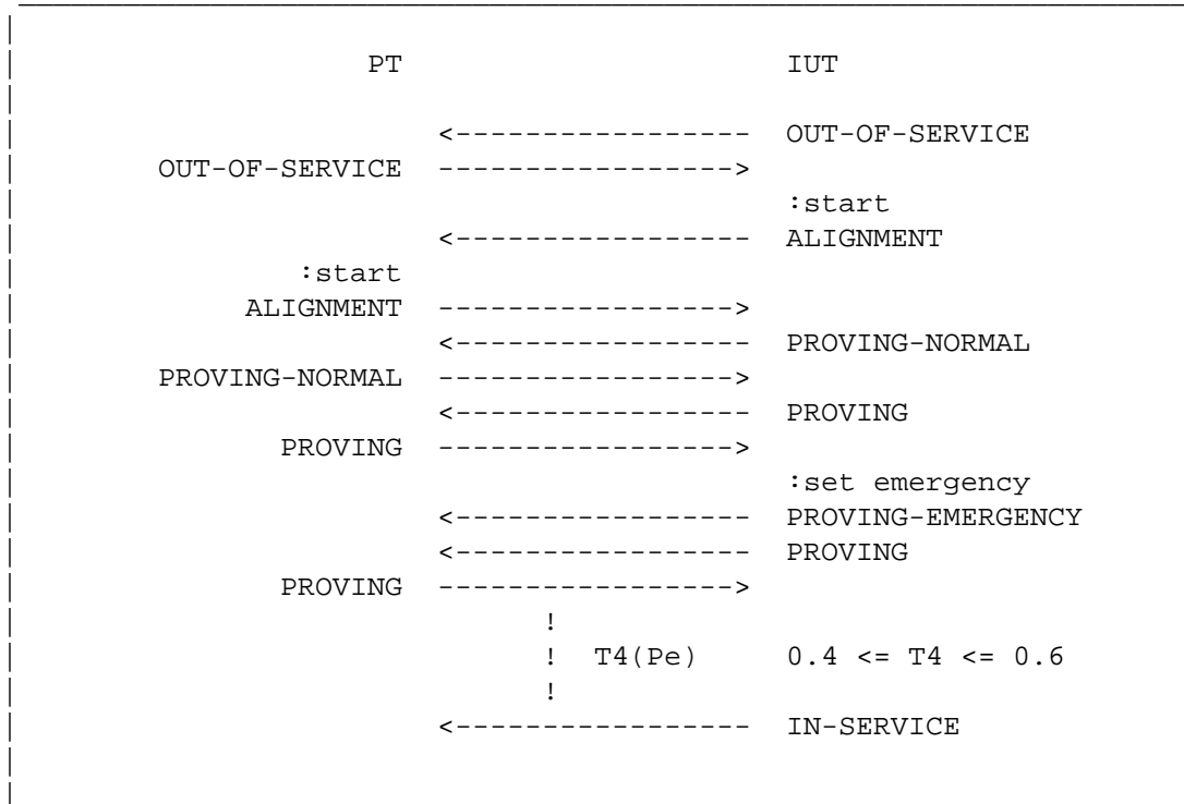
Figure 3.1.20-1. Set emergency when "aligned"
