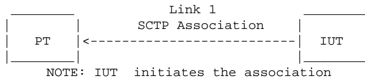
Figure 2.1-2. Test Configuration 2
