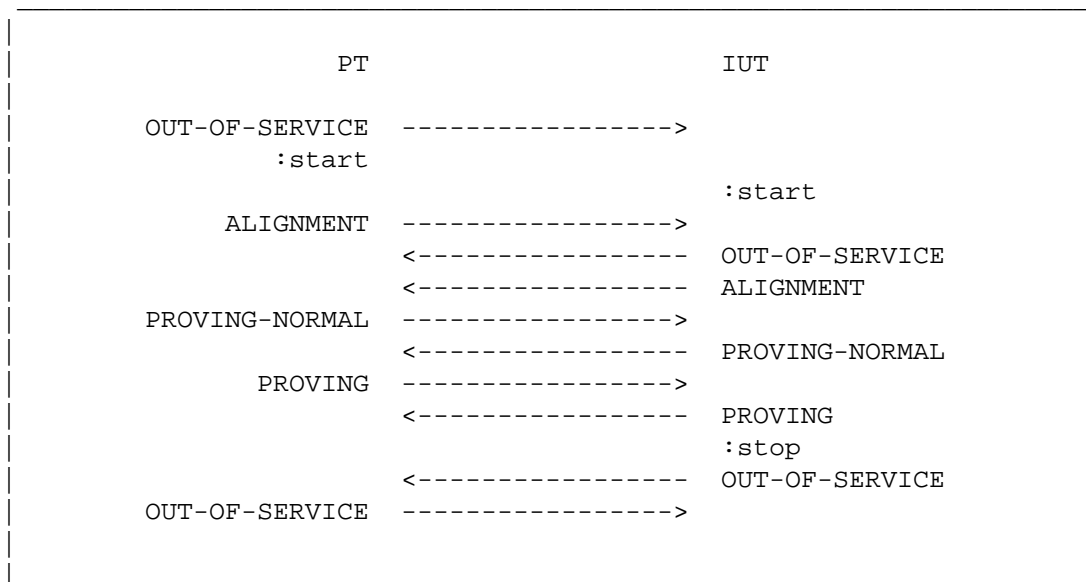
Figure 3.1.32-2. Deactivation during the proving period
