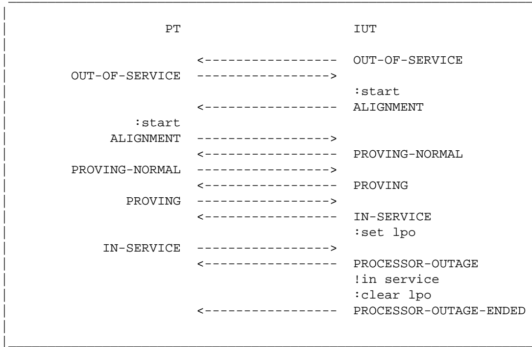
Figure 3.1.15-1. Set and clear LPO when "Aligned ready"
