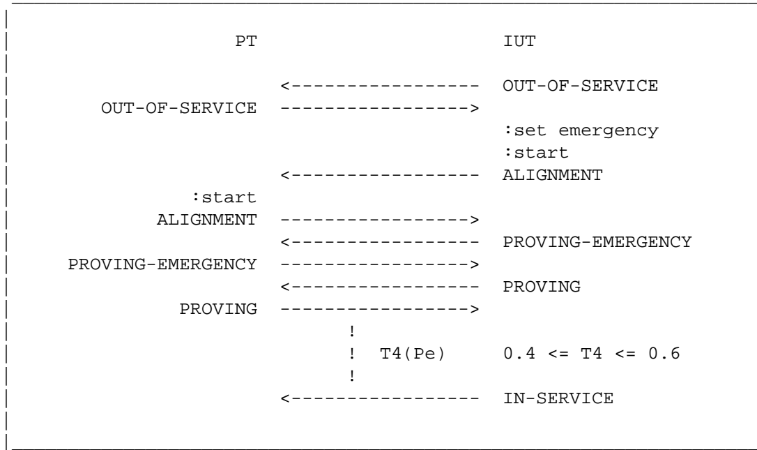
Figure 3.1.21-1. Both ends set emergency
