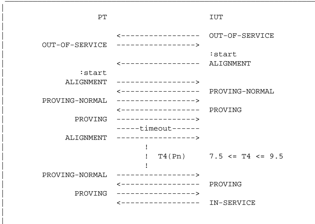
Figure 3.1.7-1. "Alignment" during normal proving
