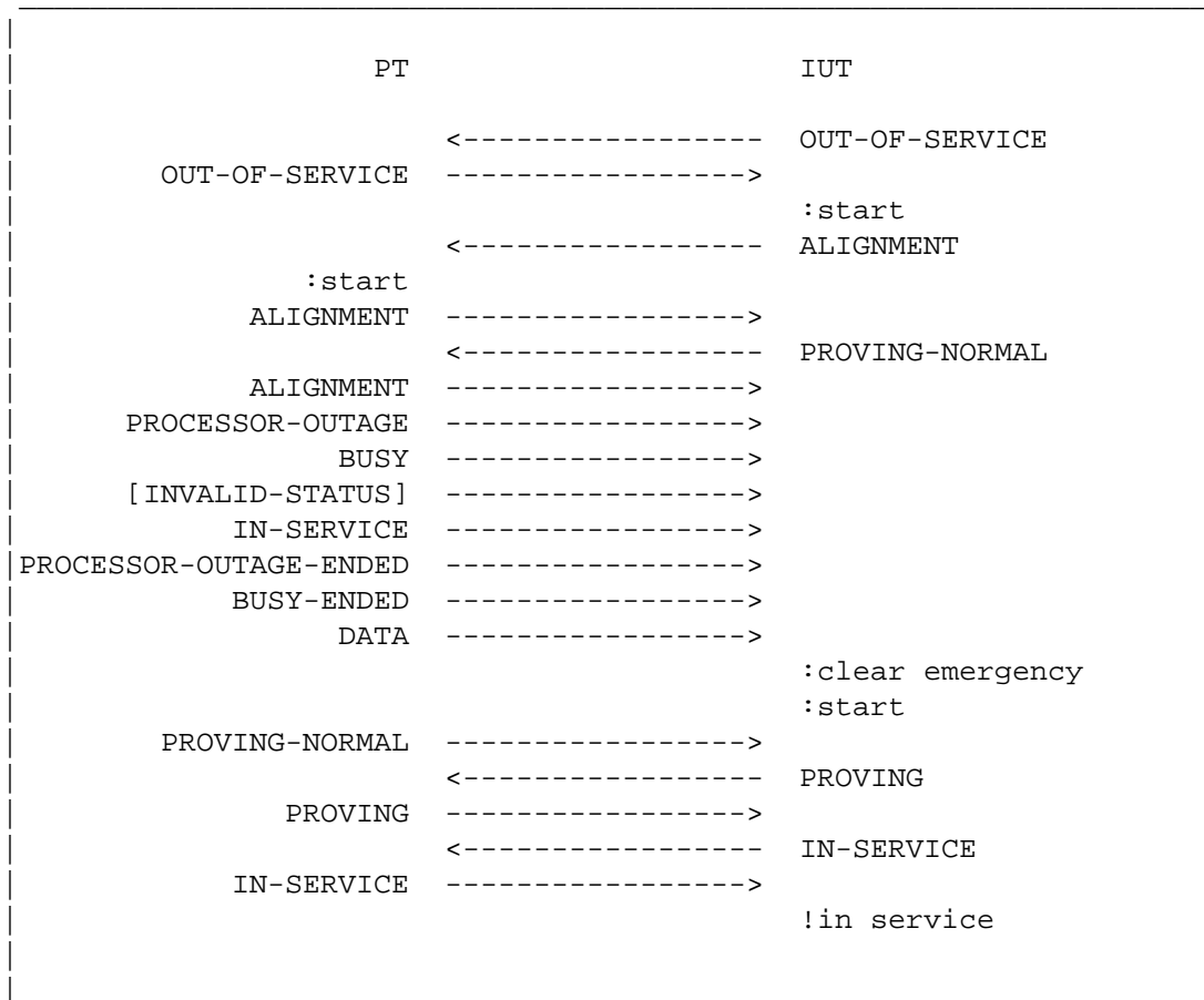
Figure 3.2.3-1. Unexpected events while "aligned"
