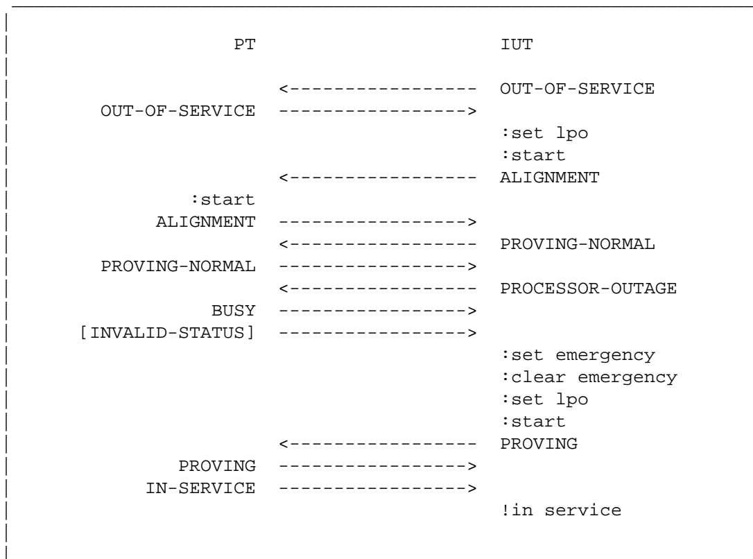
Figure 3.2.6-1. Unexpected events while "aligned not ready"
