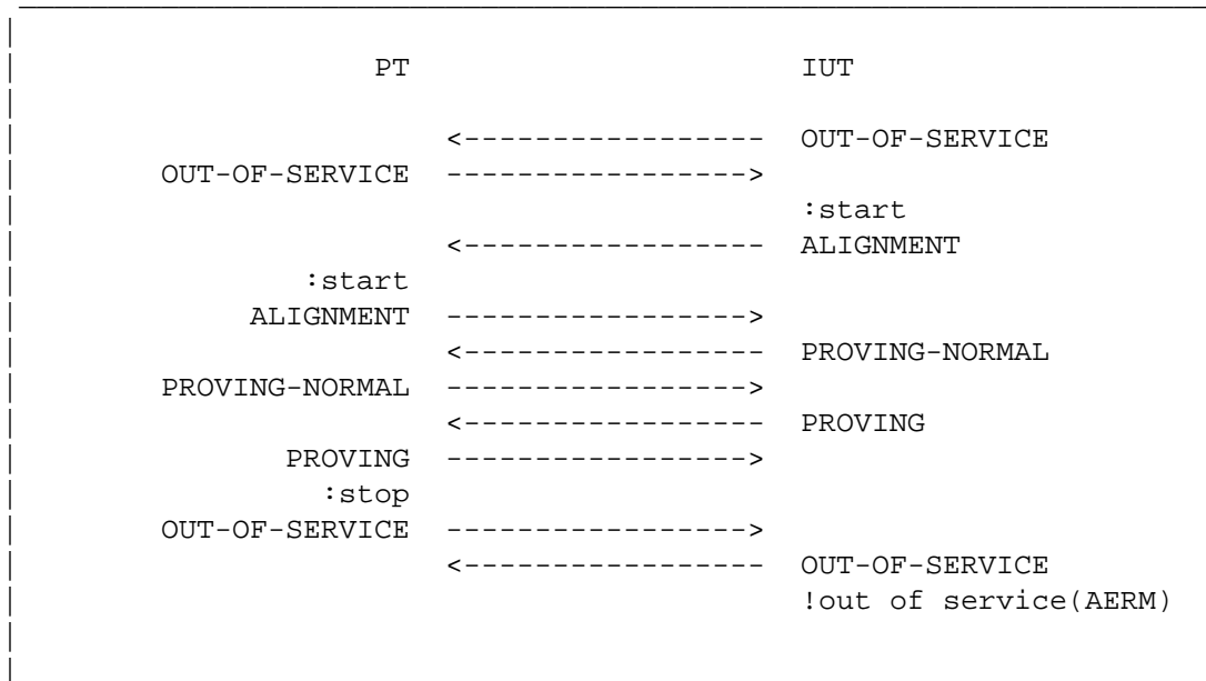
Figure 3.1.32-1. Deactivation during the proving period
