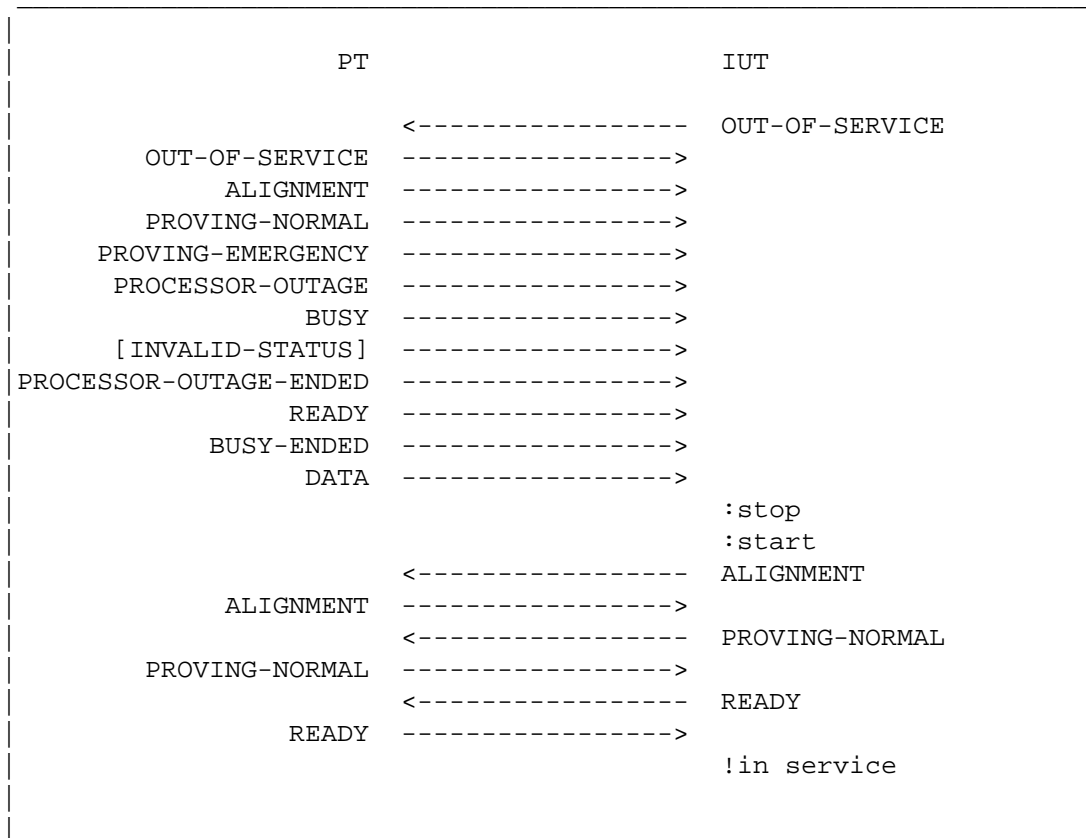
Figure 3.2.1-1. Unexpected events in the "Out of Service" State
