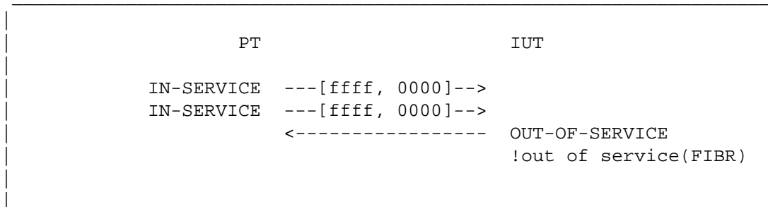
Figure 3.3.6-1. Link in service (Invalid Acks)
