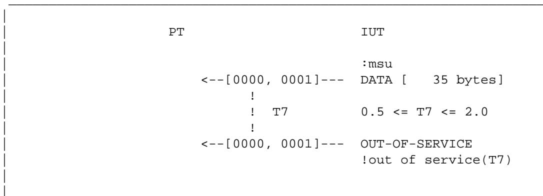
Figure 3.8.12-1. Excessive delay of acknowledgments
