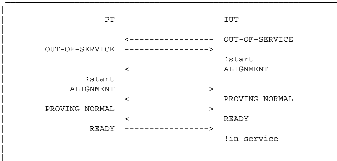
Figure 3.1.5-1. Normal alignment procedure
