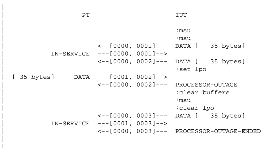
Figure 3.4.1-1. Set and clear LPO while link in service
