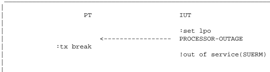
Figure 3.3.7-1. Link in processor outage (Abort)
