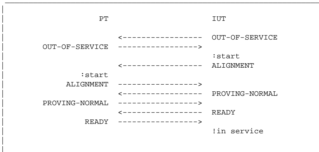
Figure 3.1.5-2. Normal alignment procedure
