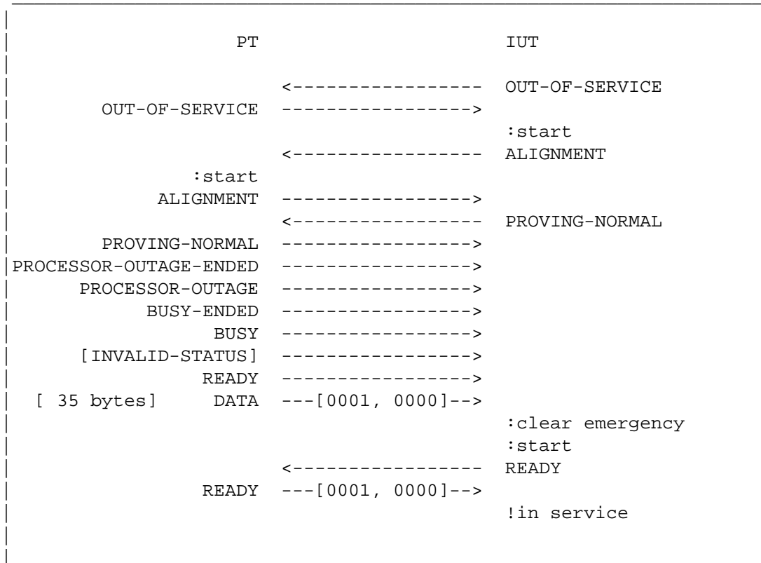
Figure 3.2.4-1. Unexpected events while "proving"
